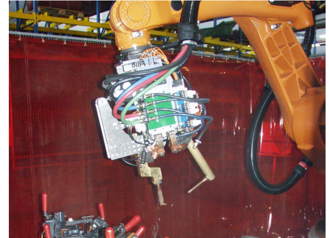
Welding tongs
