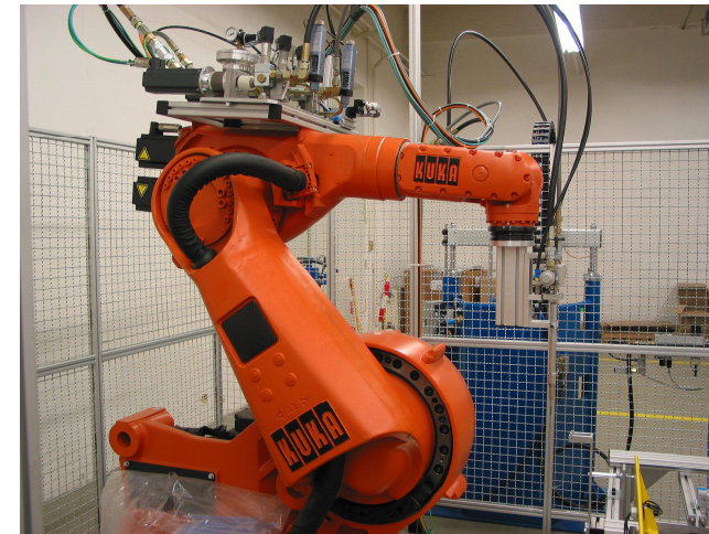
Glue feeding unit
