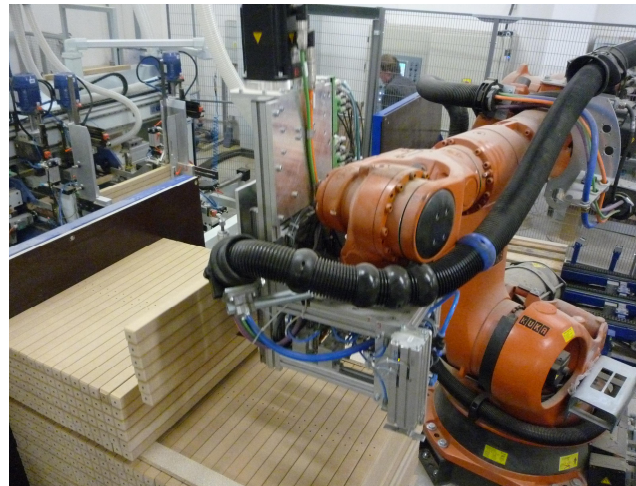
Storing the stack components on the output pallet
