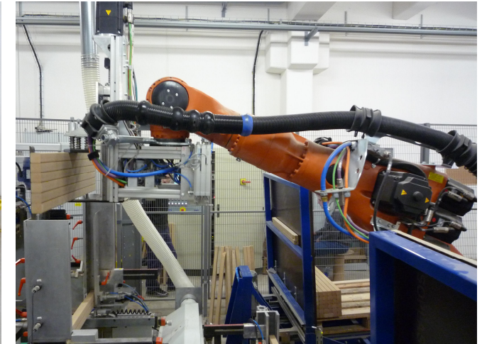
Loading stack components in the input tray woodworking machine Frontal 3S 1000 CNI of comp.COMECE
