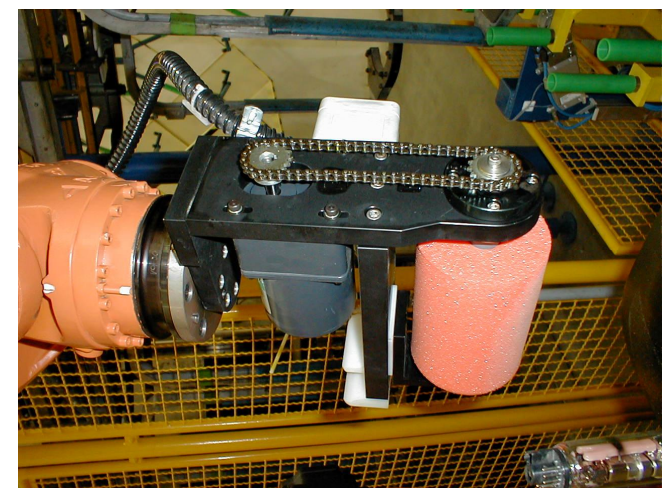
Drive of the roll
