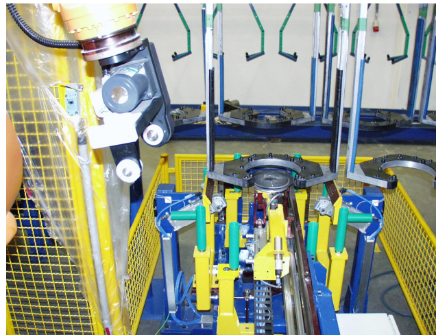
Centering unit
