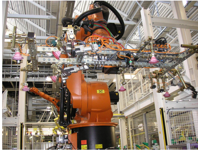
AFO 40 – grab for roof loading
