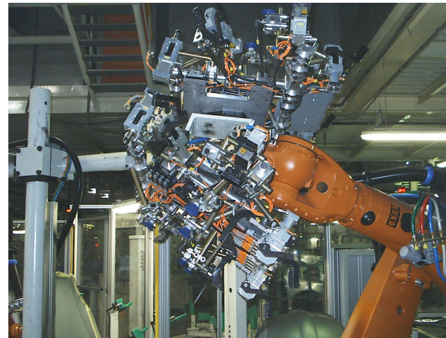
Grab of the transfer robot
