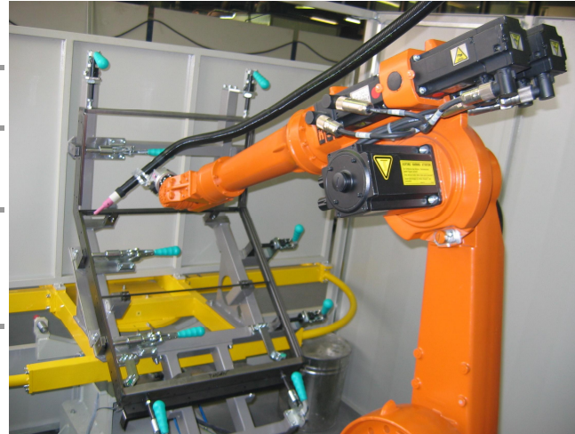
Installation of feeders and MIG torch
