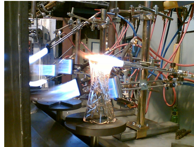
Withdrawal place from the polishing machines
