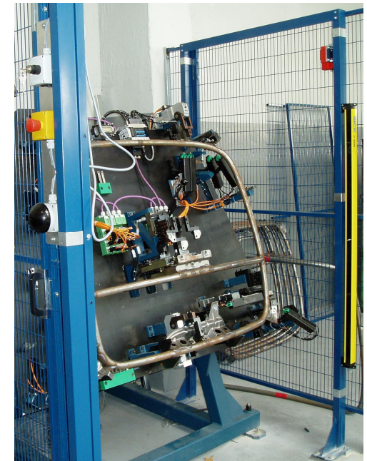
Gauging fixture
